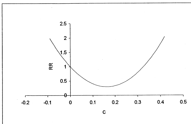
Fig. 1. Relative risk for p = 3 , n = 10 , v = 5
