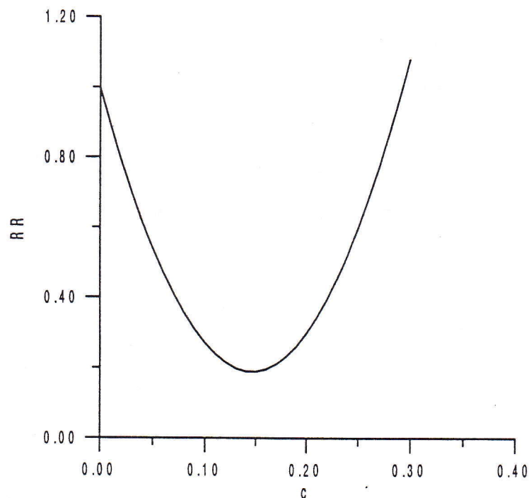
Figure 2 - Relative Risk (RR) versus c ( p = 4 , v = 5 , n = 10 and \bar{\xi}/\ddot{\xi} = 1.590451 ).
