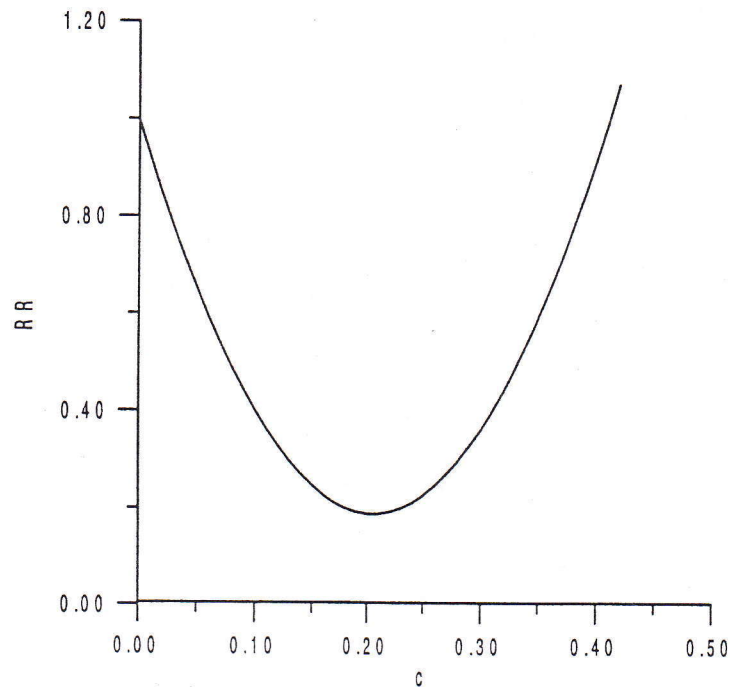
Figure 1 - Relative Risk (RR) versus c ( p = 4 , v = 5 , n = 10 and \bar{\xi}/\ddot{\xi} = 2.229844 ).
