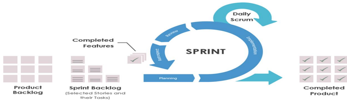
Figure 3.2: Scrum methodology
