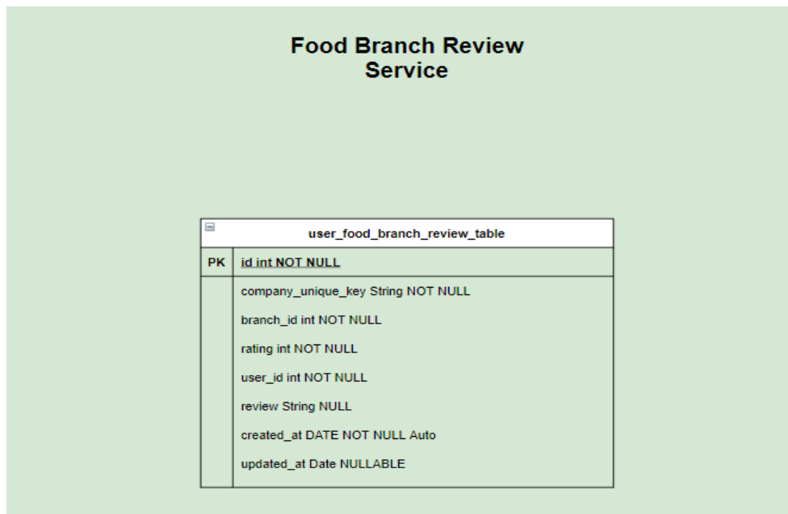
Figure 3.17: ER diagram of Food Branch Review Service
