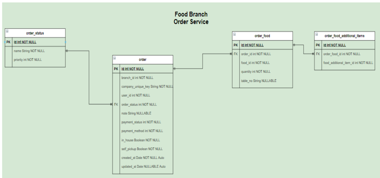
Figure 3.15: ER diagram of Food Order Service
