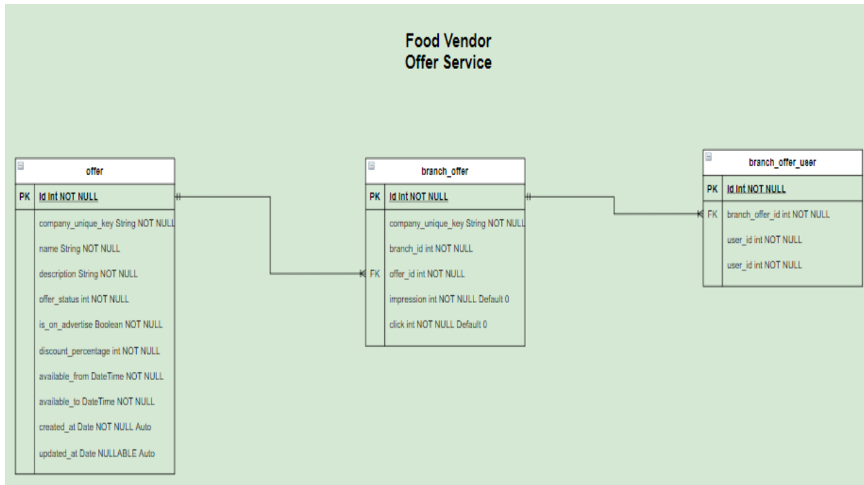
Figure 3.14: ER diagram of Food Offer Service
