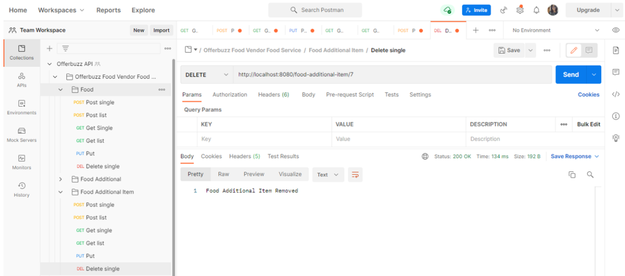
Figure 3.25: DELETE mapping
