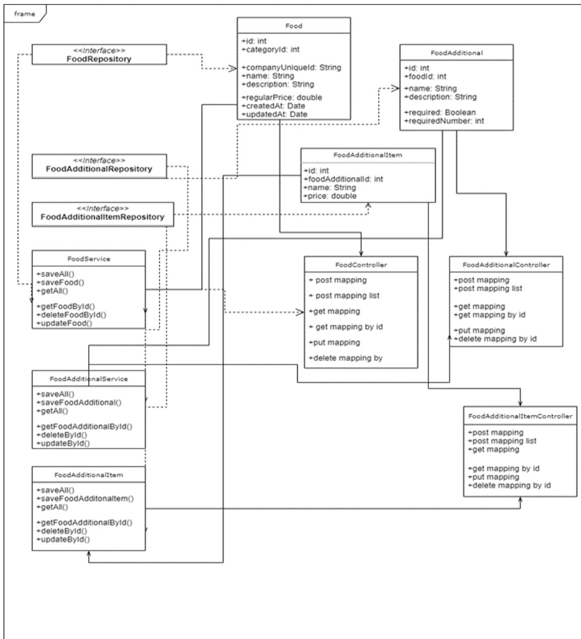
Figure 3.19: Class diagram for Food Service
