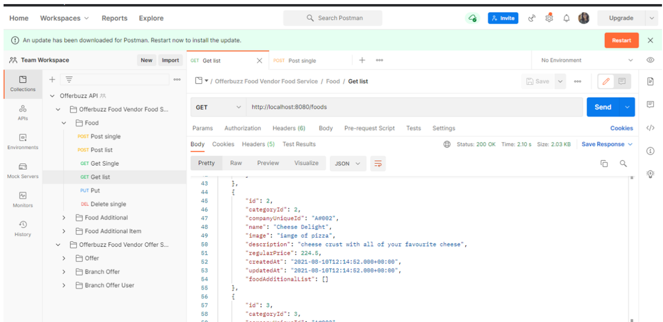
Figure 3.21: GET mapping (List)
