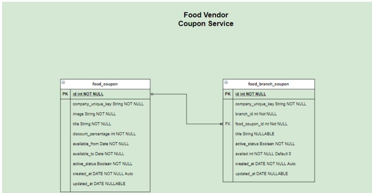
Figure 3.18: ER diagram of Food Coupon Service
