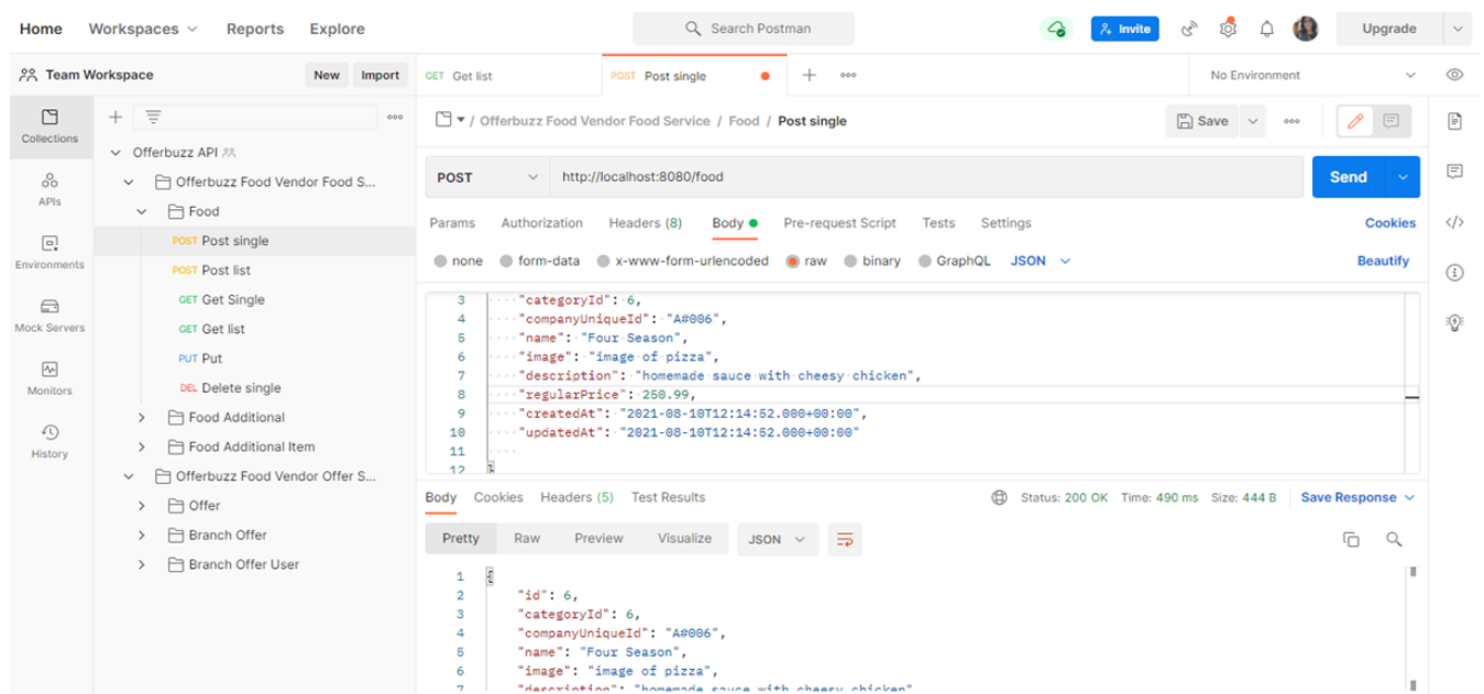
Figure 3.20: POST mapping of a service
