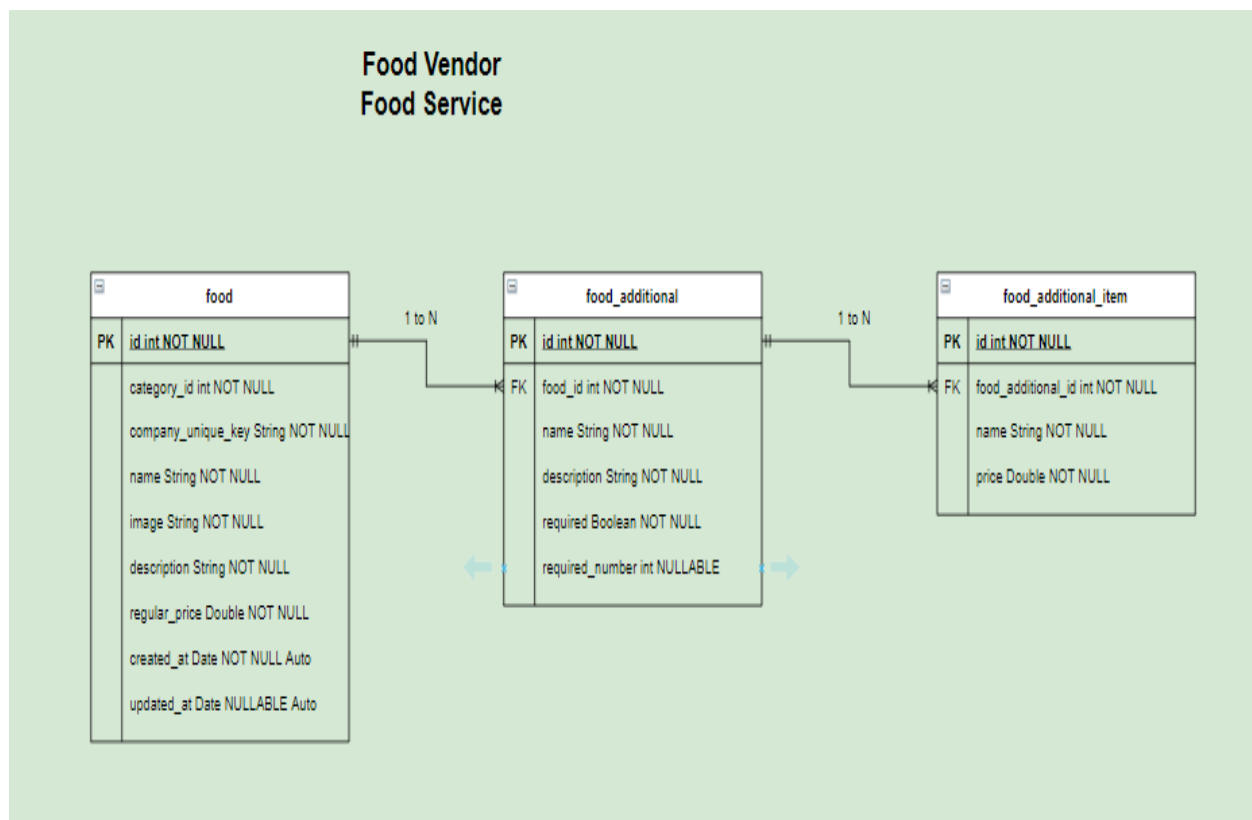
Figure 3.13: ER diagram of Food Service
