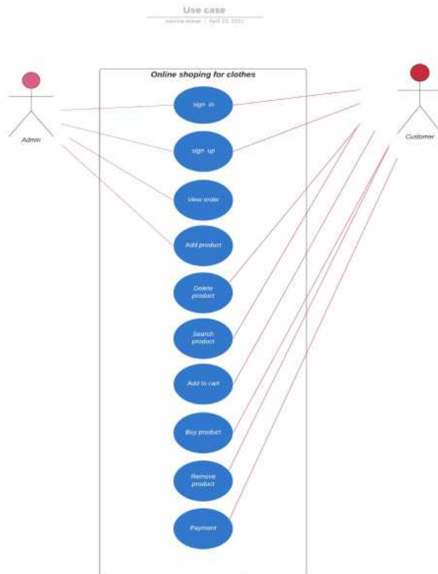
Fig 1.2: Use case diagram
